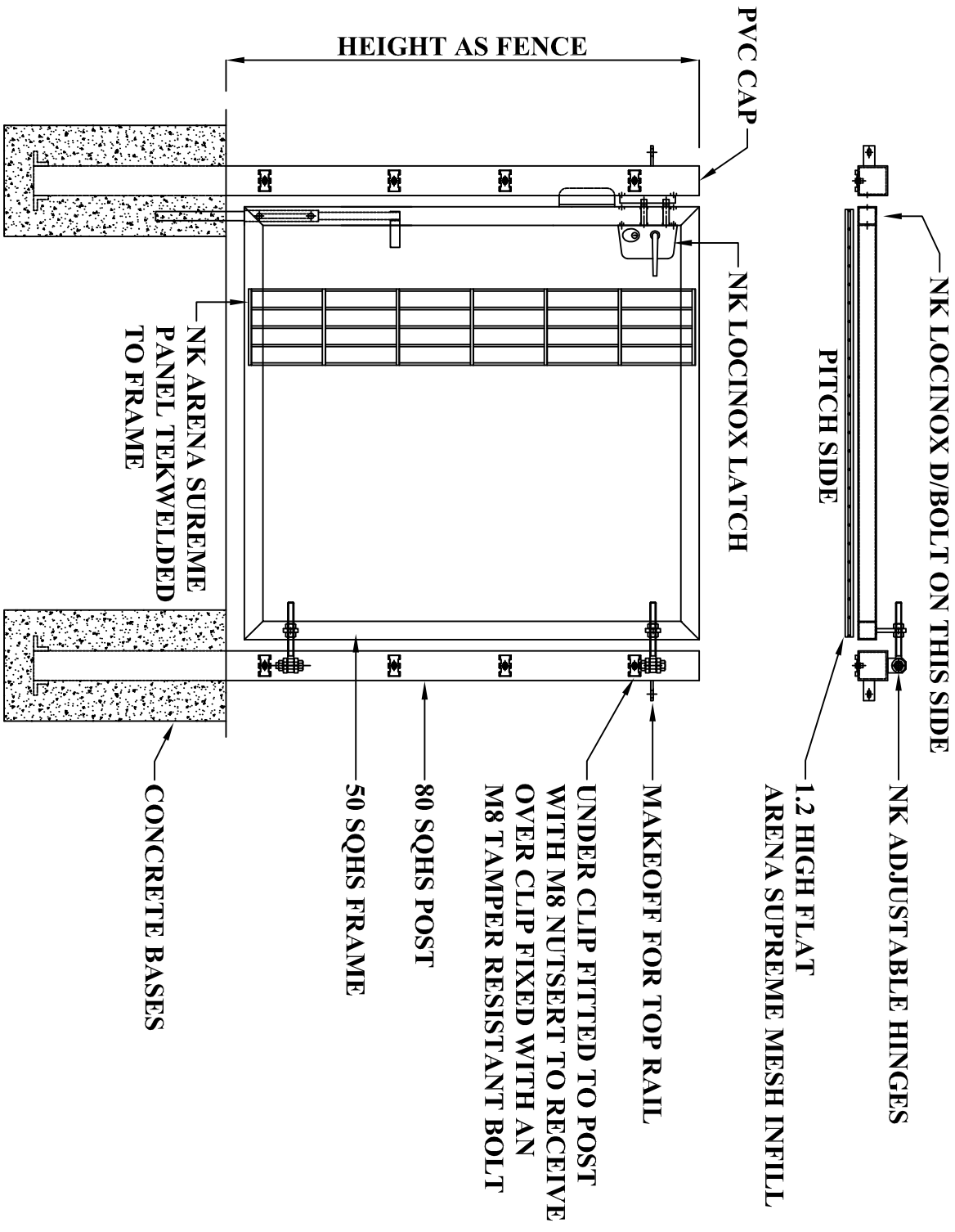
NK ARENA SPECTATOR S/L GATE - TYPICAL ELEVATION
