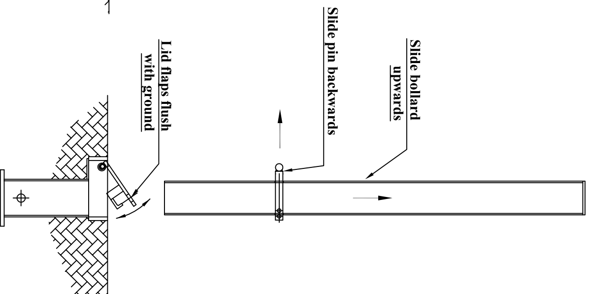
BOLLARD IN REMOVED POSITION
